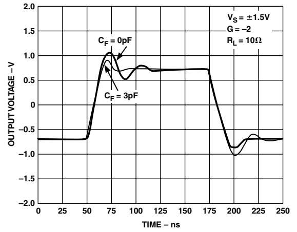
TPC 5. Large Signal Step Response
