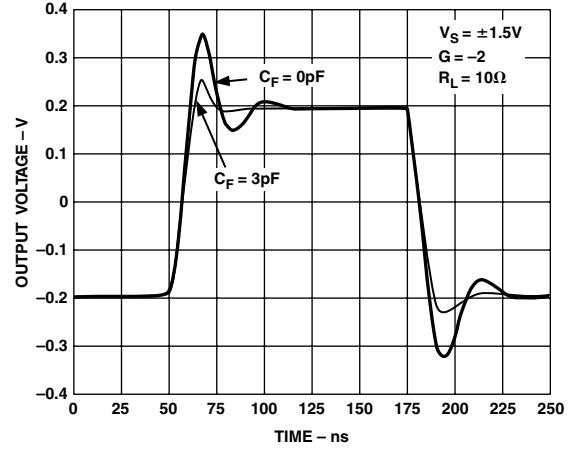
TPC 4. Small Signal Step Response
